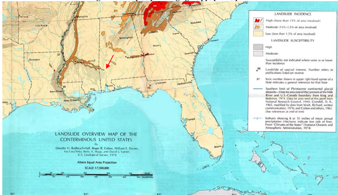
Figure 4.11 http://pubs.usgs.gov/pp/p1183/plate1.html
